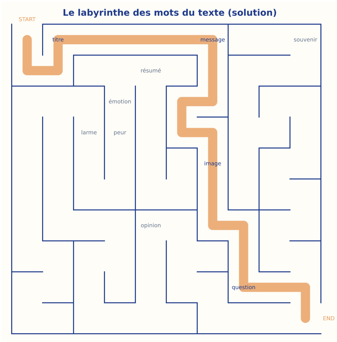
Maze solution
